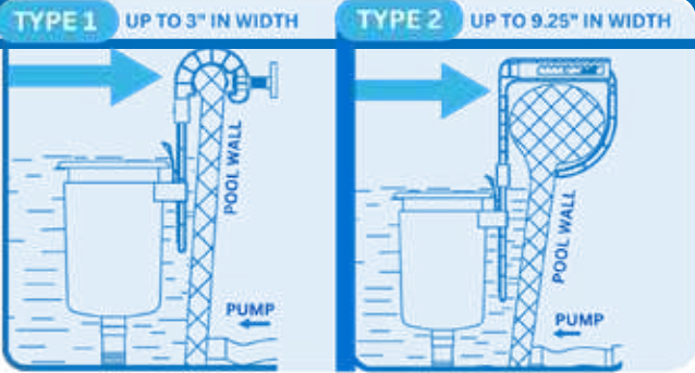
89250 Adjustable Hanging Pool Skimmer Includes two adjustable bracket options used with inflatable collars, tubular and metal frame soft-sided pools. 9" of vertical height adjustability. Case Qty: 4
